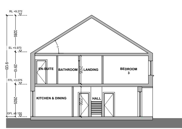
7 Section 1:200
