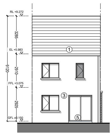
5 Rear Elevation 1:200
