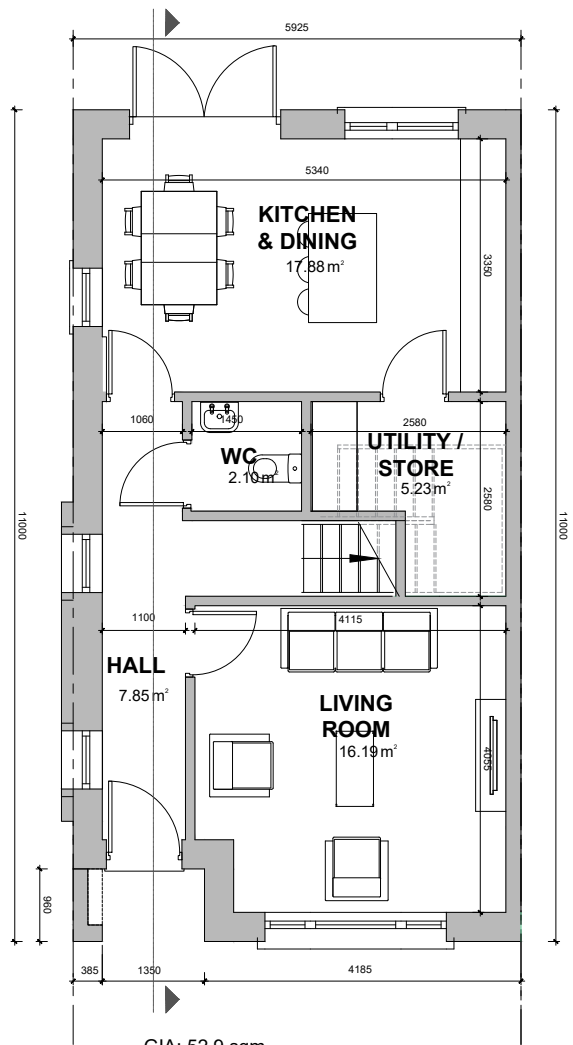
GIA: 52.9 sqm 1 Ground floor plan 1:100
