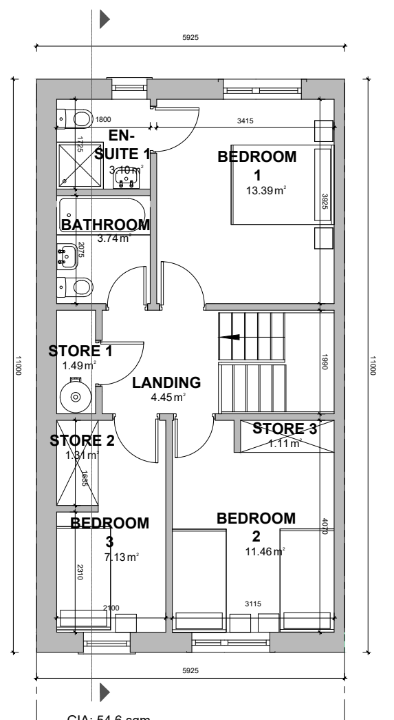
GIA: 54.6 sqm 2 First floor plan 1:100
