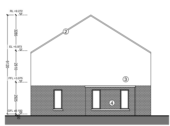
6 Side elevation 1:200
