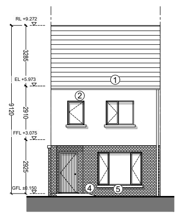
4 Front Elevation 1:200
